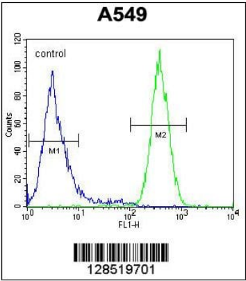
FCM/FACS (Flow Cytometry) NGRN Antibody (C-term) flow cytometric analysis of A549 cells (right histogram) compared to a negative control cell (left histogram).FITC-conjugated goat-anti-rabbit secondary antibodies were used for the analysis.
