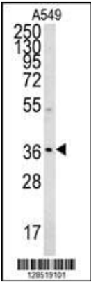
WB (Western Blot) NGRN Antibody (C-term) western blot analysis in A549 cell line lysates (35ug/lane).This demonstrates the OR52D1 antibody detected the NGRN protein (arrow).
