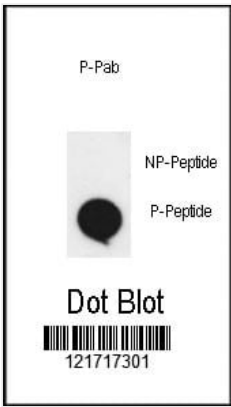
DB (Dot Blot) Dot blot analysis of anti-phospho-EphA2-pS897 Phospho-specific Pab on nitrocellulose membrane. 50ng of Phospho-peptide or Non Phospho-peptide per dot were adsorbed. Antibody working concentrations are 0.5ug per ml.
