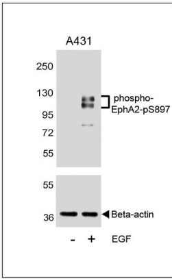
WB (Western Blot) Western blot analysis of lysates from A431 cell line, untreated or treated with EGF, 100ng/ml, using phospho-EphA2 Antibody (pS897) (upper) or Beta-actin (lower).
