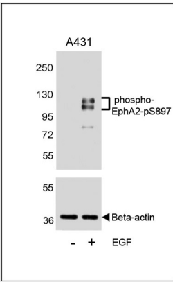
WB (Western Blot) Western blot analysis of EphA2 Antibody (pS897) Pab (RB21717) pre-incubated without(lane 1) and with(lane 2) FBS in HA cell line lysate. EphA2 Antibody (pS897) (arrow) was detected using the purified Pab(Kindly provided by Dr. John Wu).
