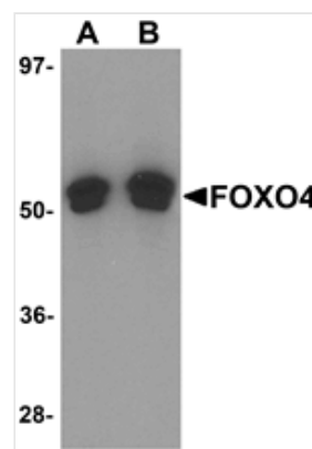
WB (Western Blot) Western blot analysis of FOXO4 in A-20 cell lysate with FOXO4 antibody at (A) 0.5 and (B) 1 ug/mL.
