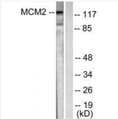
WB (Western Blot) Western blot analysis of extracts from 293 cells, using MCM2 antibody.
