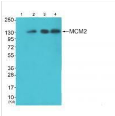
WB (Western Blot) Western blot analysis of extracts from 3T3 cells (Lane 2), k562 cells (Lane 3) and HepG2 cells (Lane 4), using MCM2 antibody. The lane on the left is treated with synthesized peptide.
