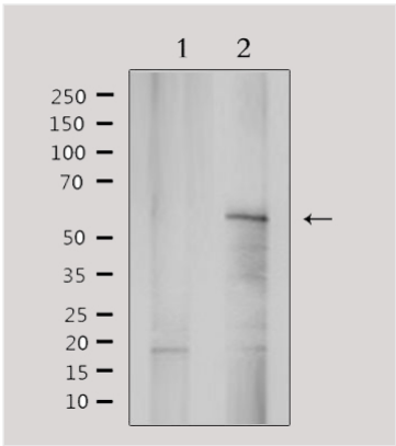
WB (Western Blot) Western blot analysis of extracts from 293, using YTHDF1 Antibody.
