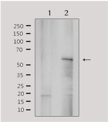
WB (Western Blot) Western blot analysis of extracts from rat brain, using YTHDF1 Antibody. Lane 1 was treated with the antigen-specific peptide.
