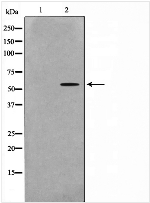
WB (Western Blot) Western blot analysis on 293 cell lysate using YTHDF1 Antibody. The lane on the left is treated with the antigen-specific peptide.
