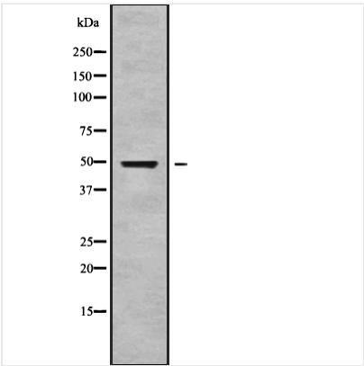
WB (Western Blot) Western blot analysis of PSG3 using HepG2 whole cell lysates
