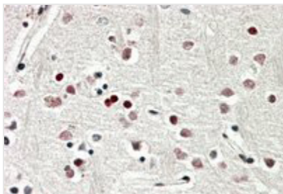
IHC (Immunohistochemistry)
