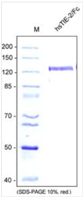
SDS-PAGE SDS-PAGE analysis of recombinant human soluble TIE-2/Fc produced from insect cells. Sample was loaded in 10% SDS-polyacrylamide gel under reducing condition and stained with Coomassie blue.
